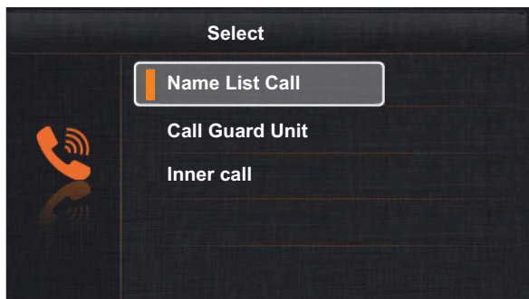
Selection screen
