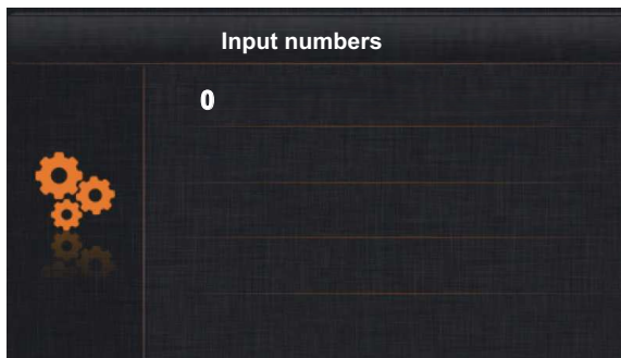
Editing screen
