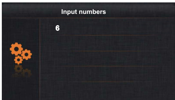
Editing screen
