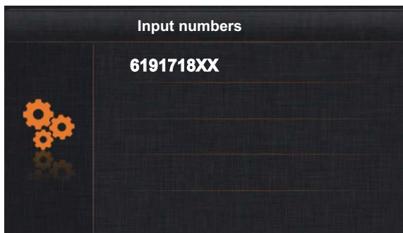
Editing screen
